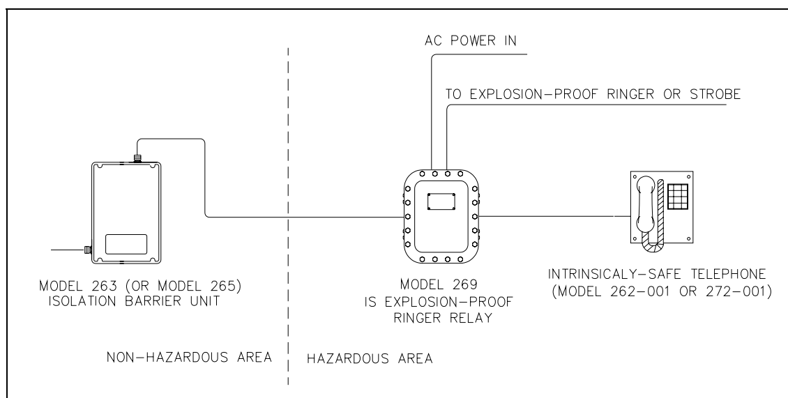
Figure 3. An Alternative Explosion-proof Ringer Placement using a Model 269 I.S. Explosion-Proof Ringer Relay
