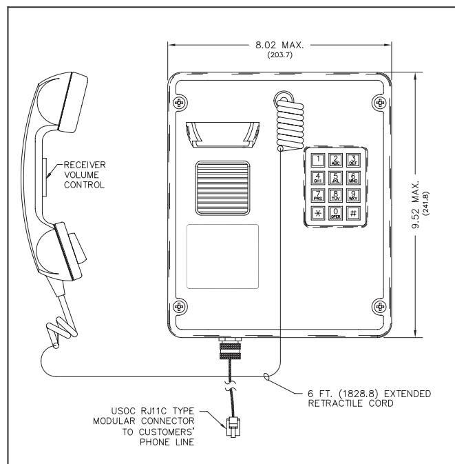
Figure 1. Model 262-001 Intrinsically-Safe Telephone
