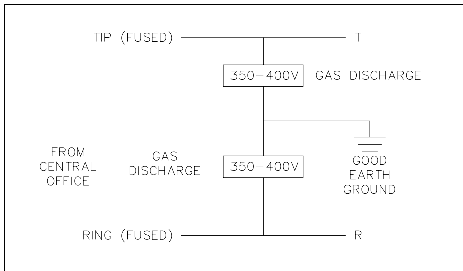
Figure 4. Example of Lightning Protection Design
